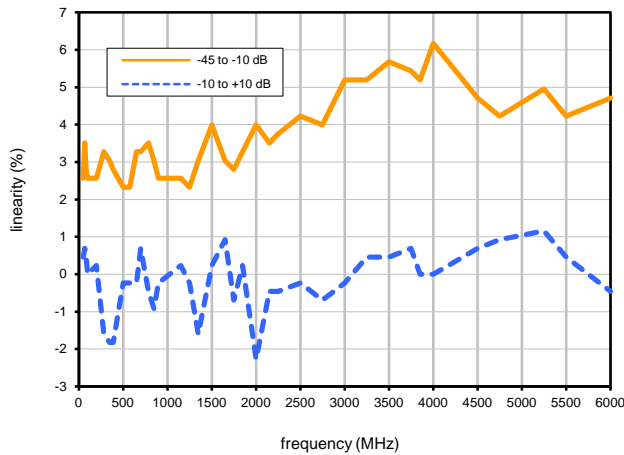
LINEARITY @ 25°C
