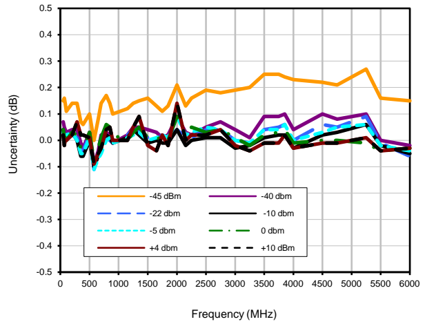
UNCERTAINTY OF POWER MEASUREMENT CW SIGNAL @ 25°C
