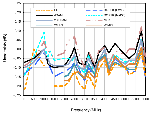
UNCERTAINTY OF POWER MEASUREMENT MODULATED SIGNAL @ 25°C
