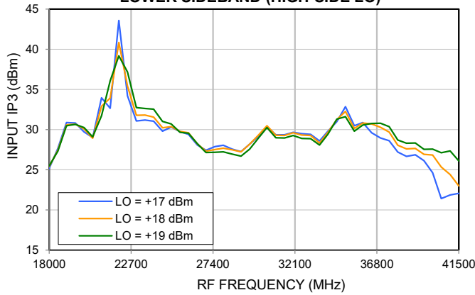
INPUT IP3 (I) @ FIXED IF = 3 GHz LOWER SIDEBAND (HIGH-SIDE LO)
