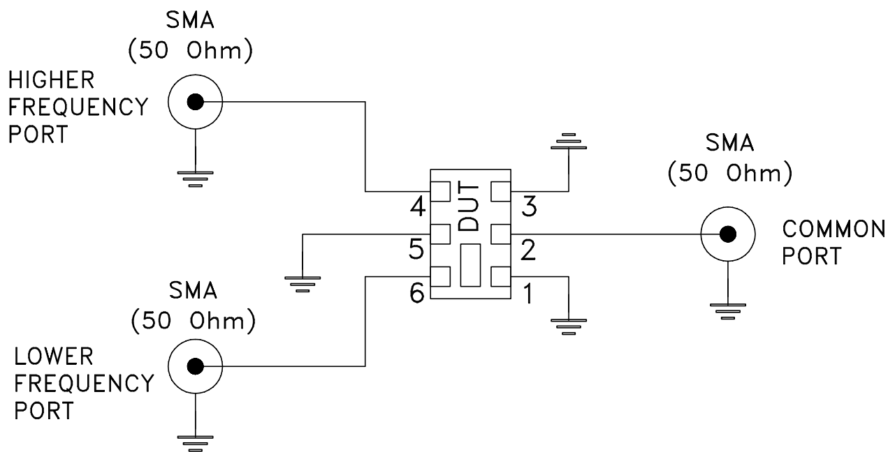
Schematic Diagram
