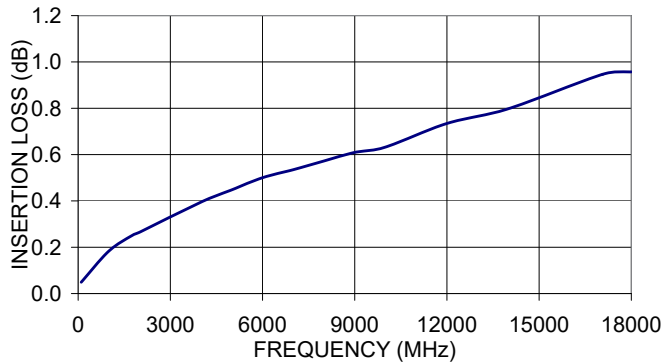
086-9SBSM+ INSERTION LOSS
