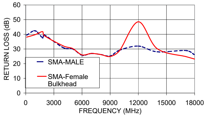
086-9SBSM+ RETURN LOSS
