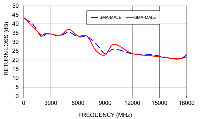
141-32SM+ RETURN LOSS
