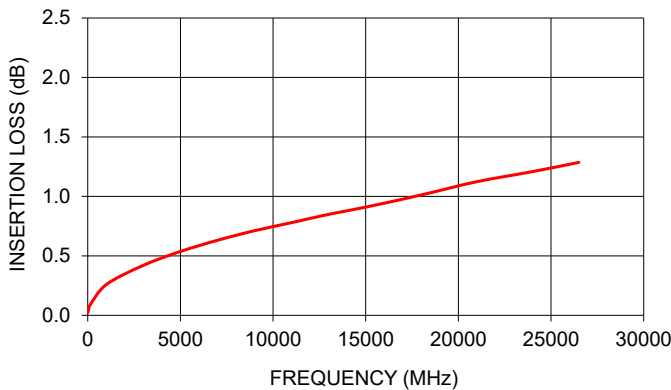
FL086-12-35M+ INSERTION LOSS
