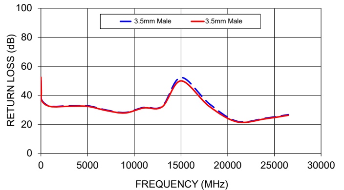
FL086-12-35M+ RETURN LOSS
