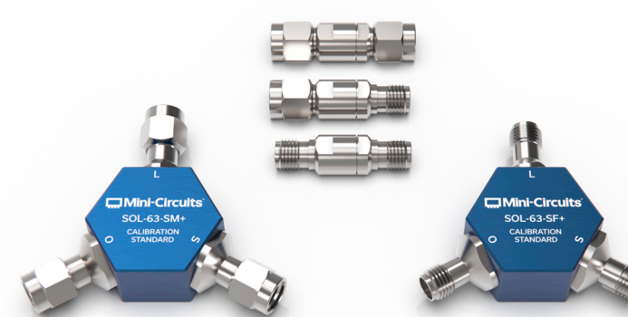
Figure 1: SMA KSOLT-63-S+ kit, including SOL (f & m) and Thru (f<math>\leftrightarrow</math>f, f<math>\leftrightarrow</math>m, m<math>\leftrightarrow</math>m) standards
