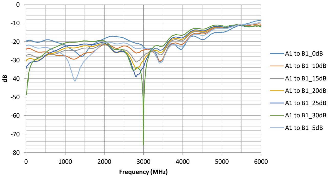
Input Return Loss (Port A1)
