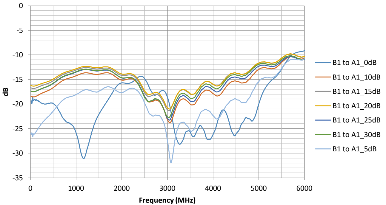
Output Return Loss (Port B1)
