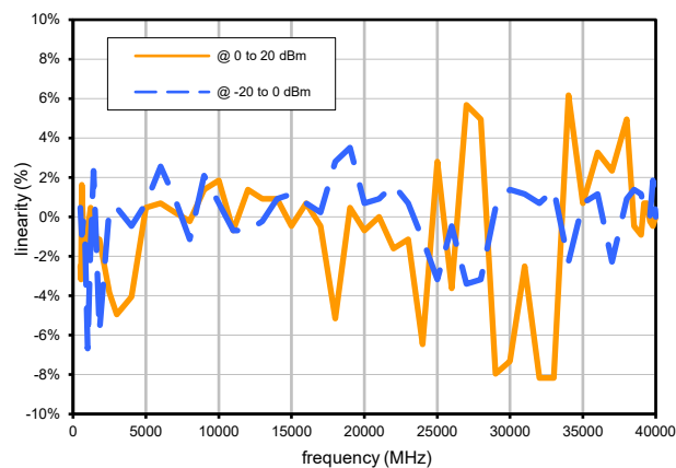
LINEARITY @ 25°C
