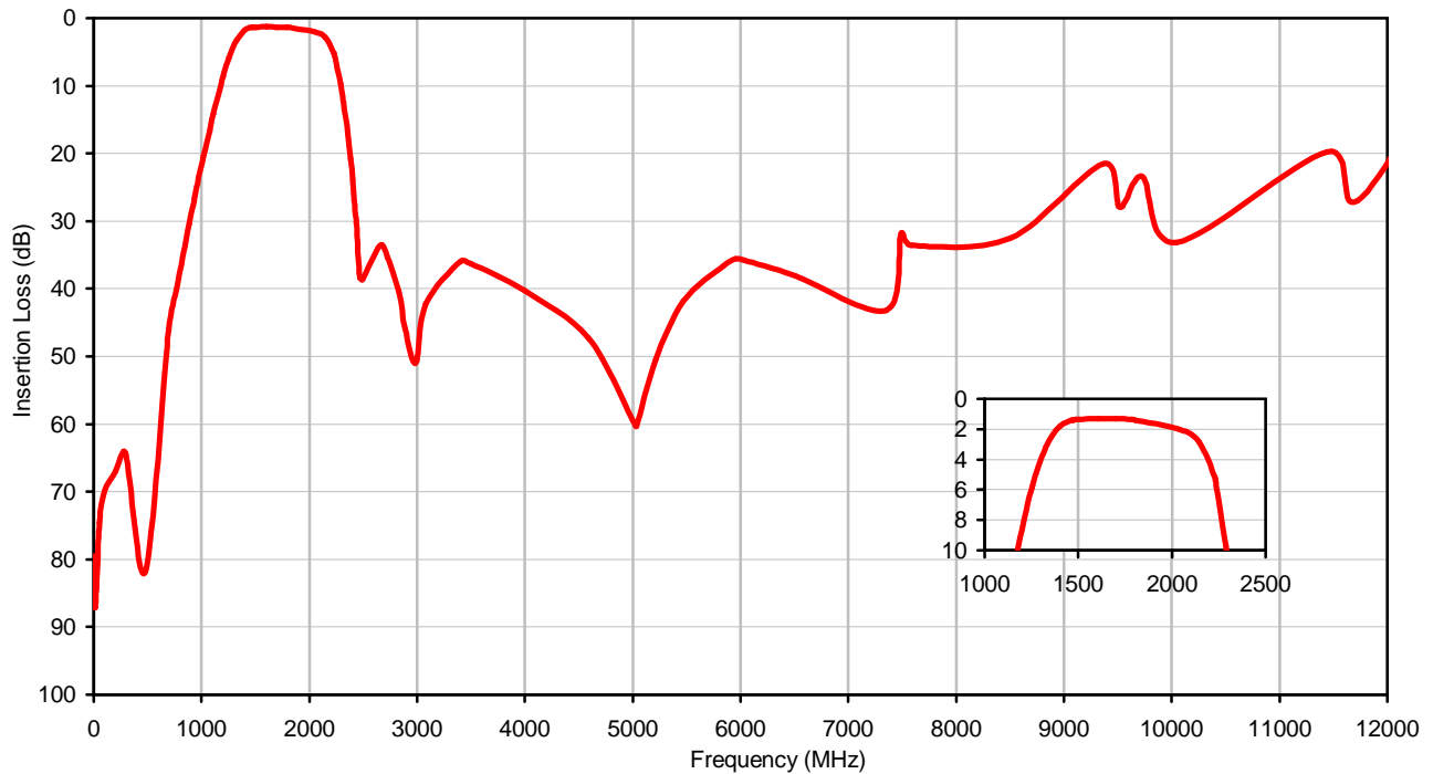
Insertion Loss
