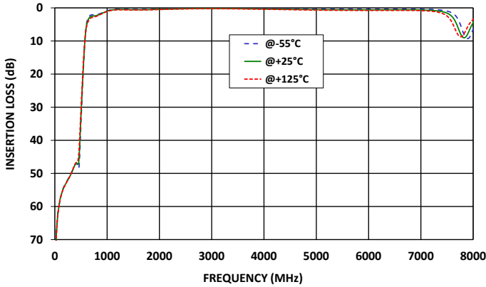
HFCG-650+ INSERTION LOSS
