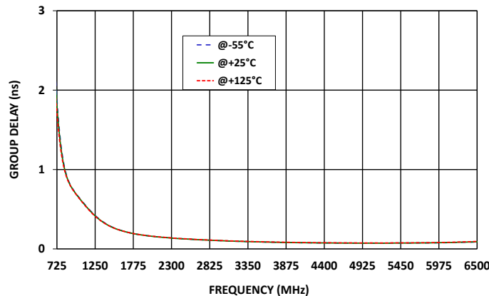
HFCG-650+ GROUP DELAY
