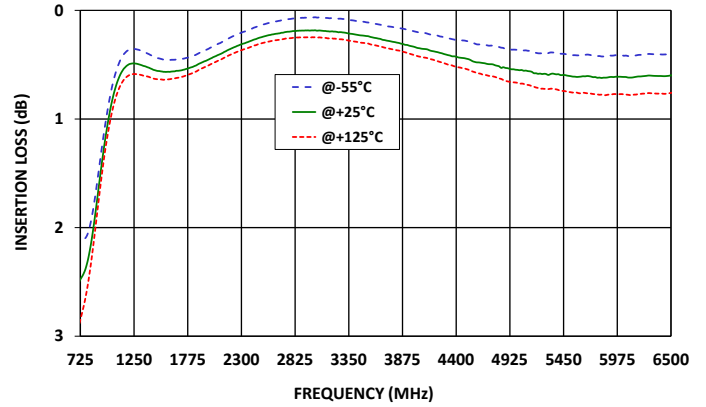
HFCG-650+ INSERTION LOSS (Zoomed)
