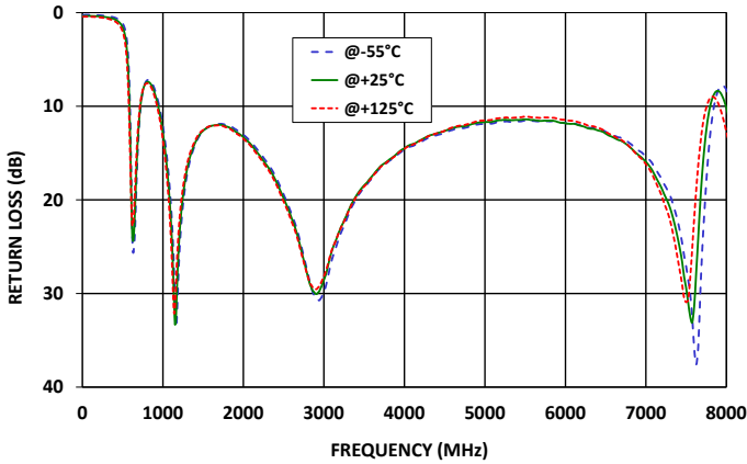
HFCG-650+ RETURN LOSS
