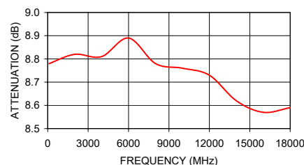
BW-S9W5+ ATTENUATION
