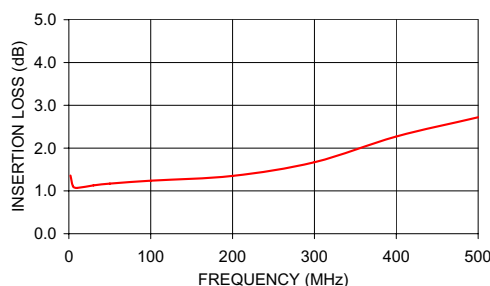
TCM8-1 INSERTION LOSS
