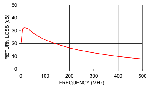
TCM8-1 INPUT RETURN LOSS
