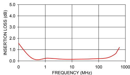
TMO-2-1+ INSERTION LOSS
