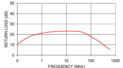
TMO-2-1+ INPUT RETURN LOSS
