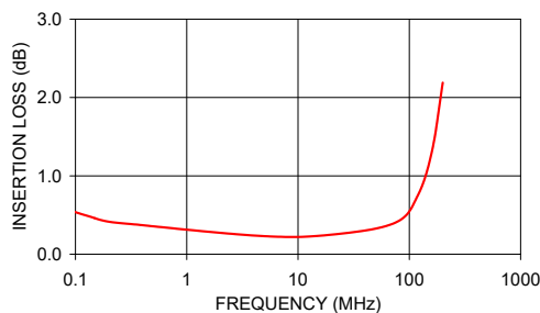
TMO-4-6+ INSERTION LOSS
