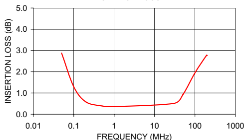
TT4-1-KK81 INSERTION LOSS
