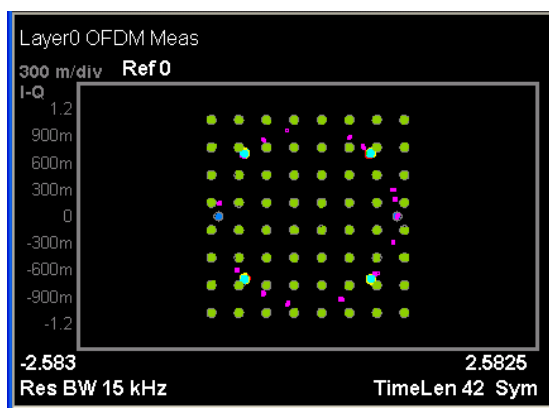
Figure 3 EVM Plot at Output Power of +14.95 dBm
