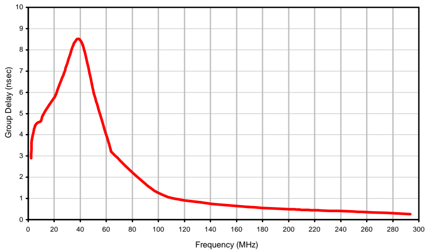
Group Delay
