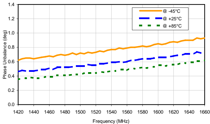
Phase Unbalance vs. Temperature
