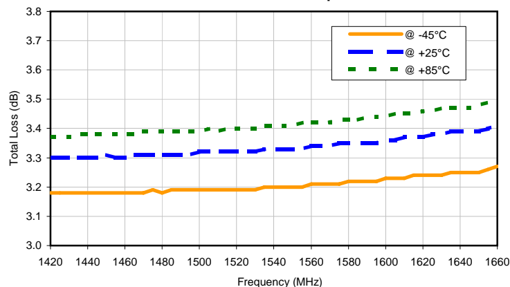
Total Loss S-1 vs. Temperature
