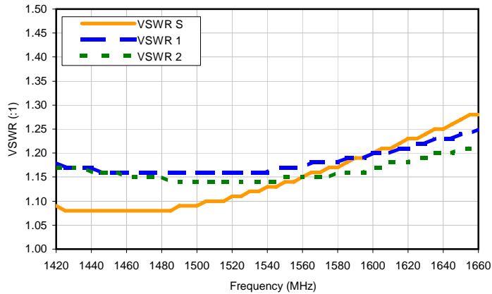
VSWR @ 25°C
