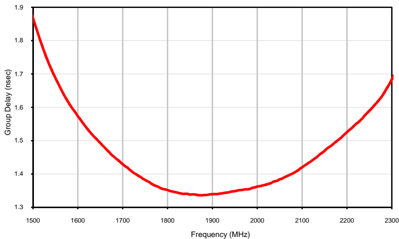
Group Delay
