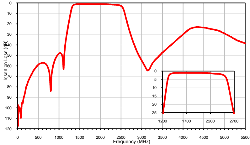
Insertion Loss
