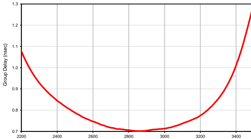
Group Delay
