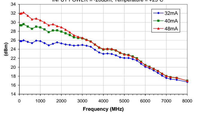
OUTPUT POWER at 1dB Compression vs. CURRENT
