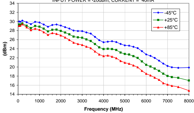
OUTPUT POWER at 1dB Compression vs. TEMPERATURE
