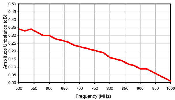
Amplitude Unbalance
