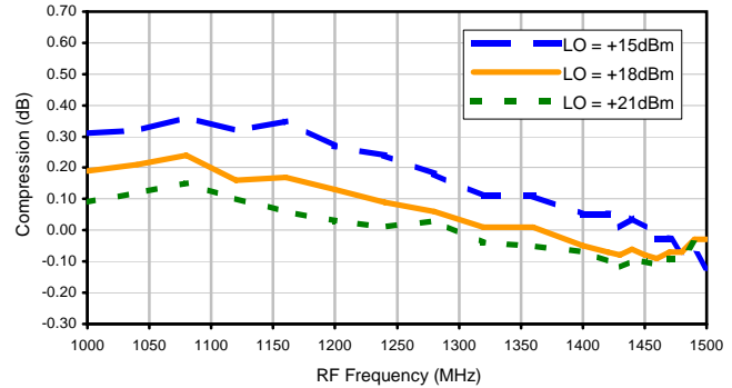
COMPRESSION @ RF=+11dBm
