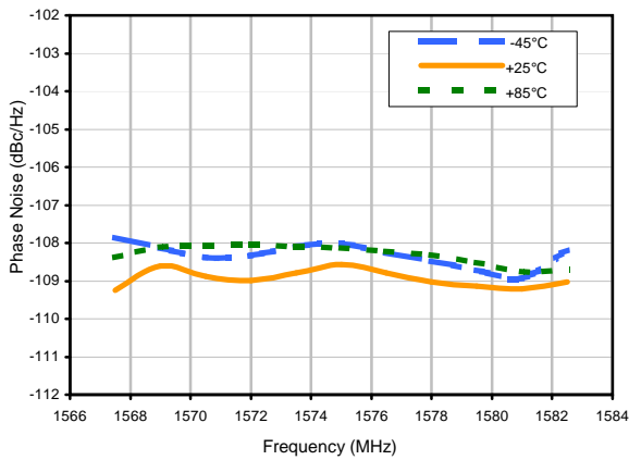
Phase Noise @ 10 kHz offset
