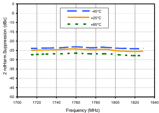
2nd Harmonics Vs Frequency
