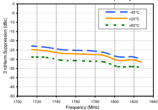
3rd Harmonics Vs Frequency
