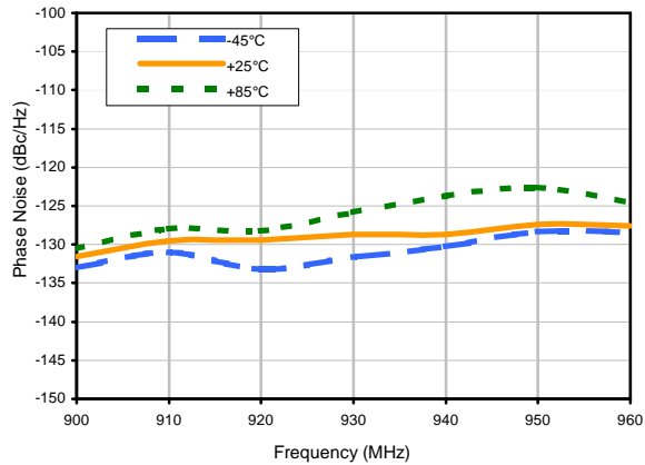
Phase Noise @ 100 kHz offset
