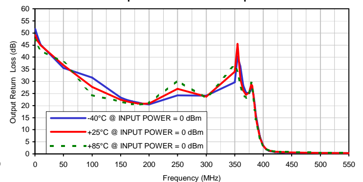
Output Return Loss vs. Temperature
