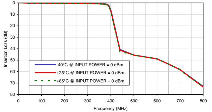
Insertion Loss vs. Temperature (Pass band)
