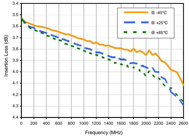
Insertion Loss S-1 vs. TEMPERATURE
