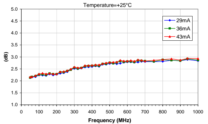
Noise Figure vs. CURRENT
