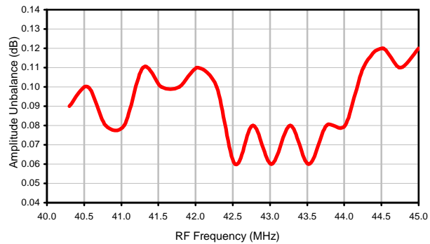
Amplitude Unbalance
