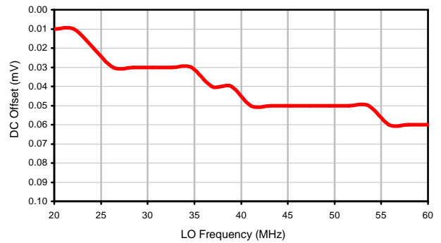
DC Offset
