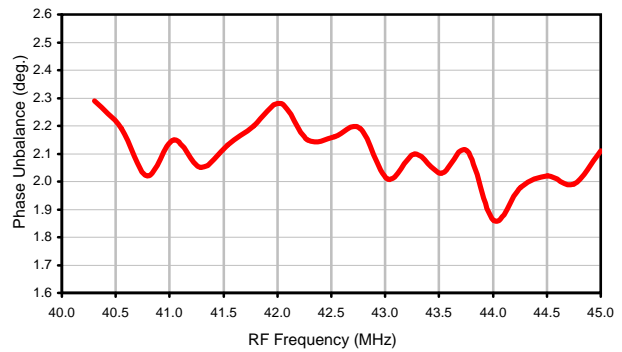
Phase Unbalance
