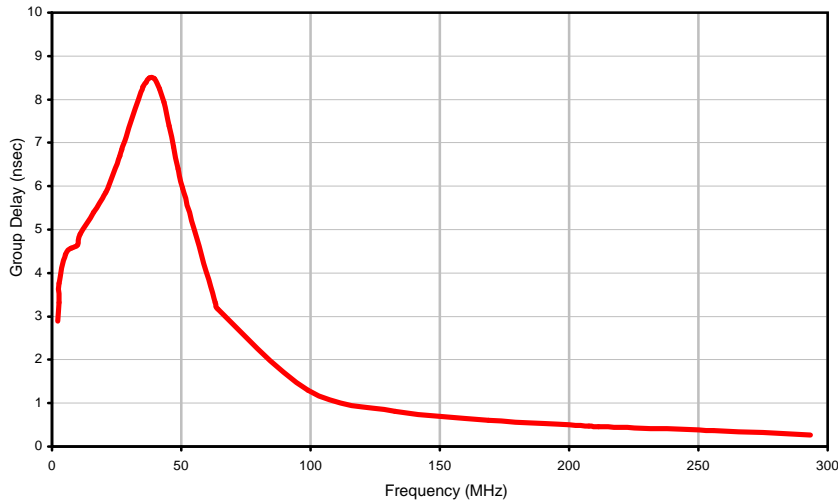
Group Delay
