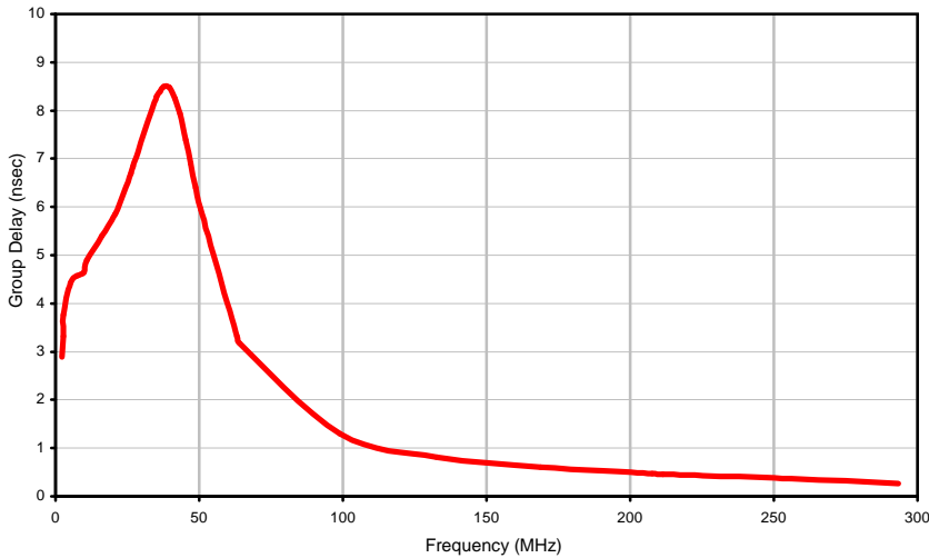
Group Delay
