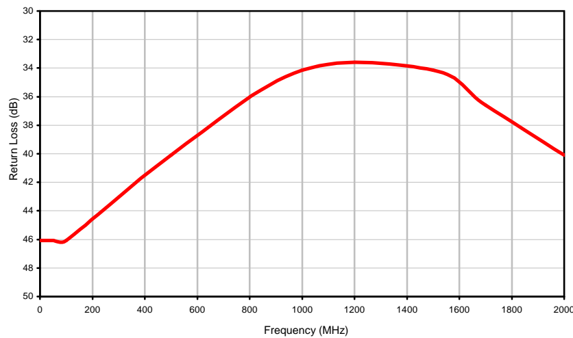
SMA-Female Return Loss
