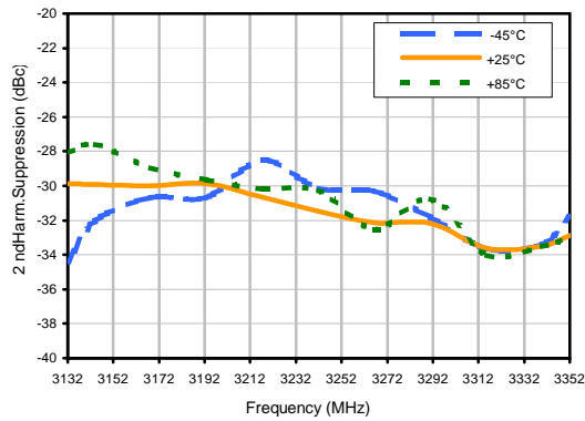
2nd Harmonics Vs Frequency
