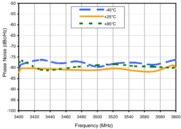
Phase Noise @ 100 Hz offset
