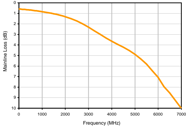
Insertion Loss
