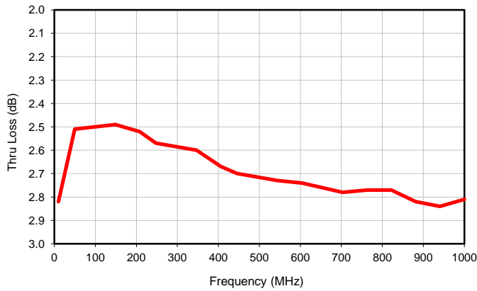
Thru Loss
