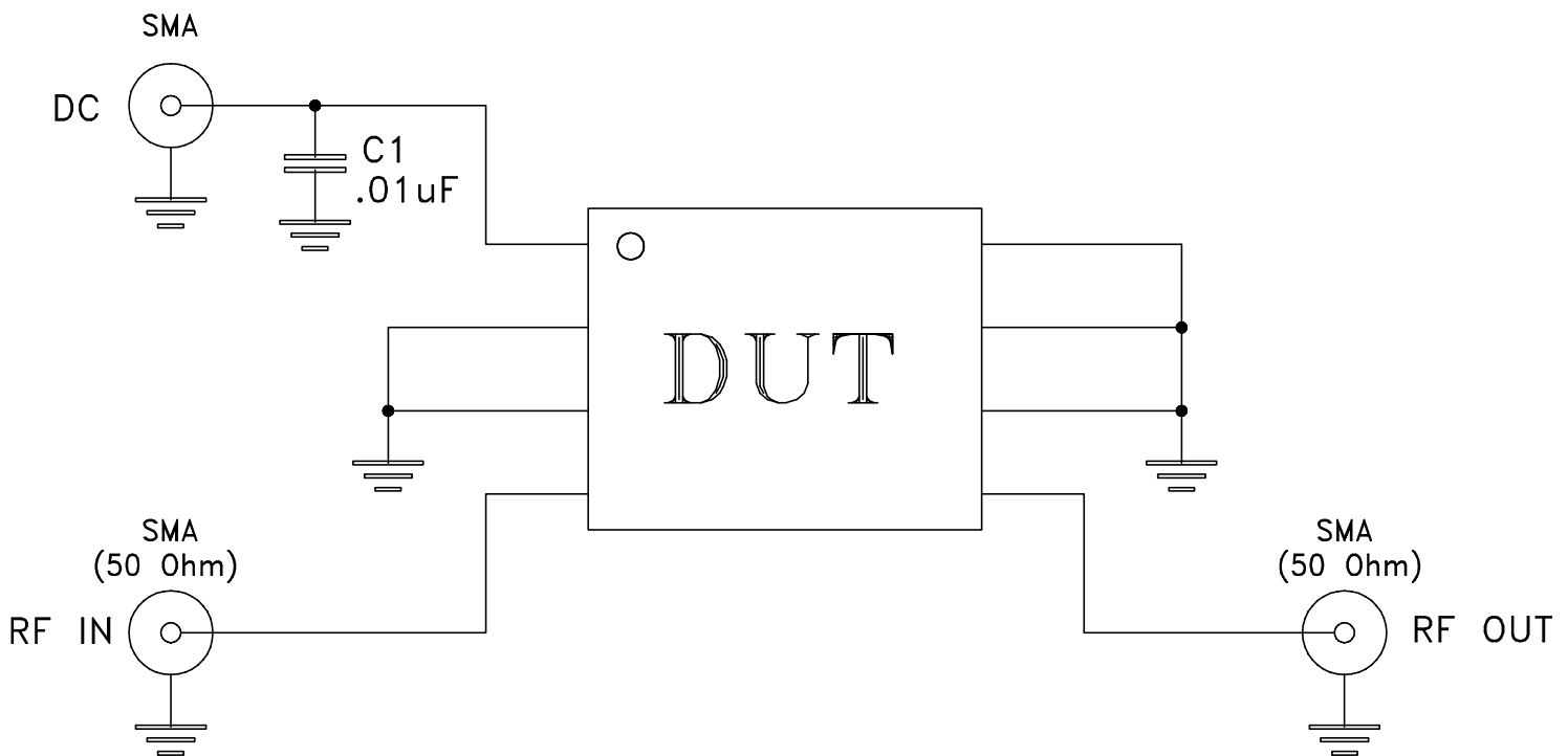
Schematic Diagram
