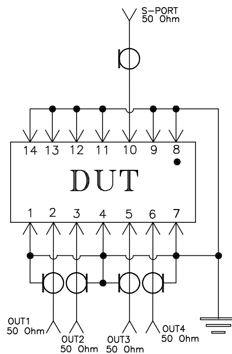
Schematic Diagram
