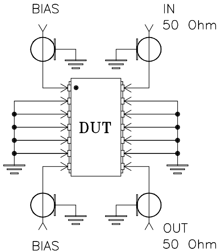
Schematic Diagram
