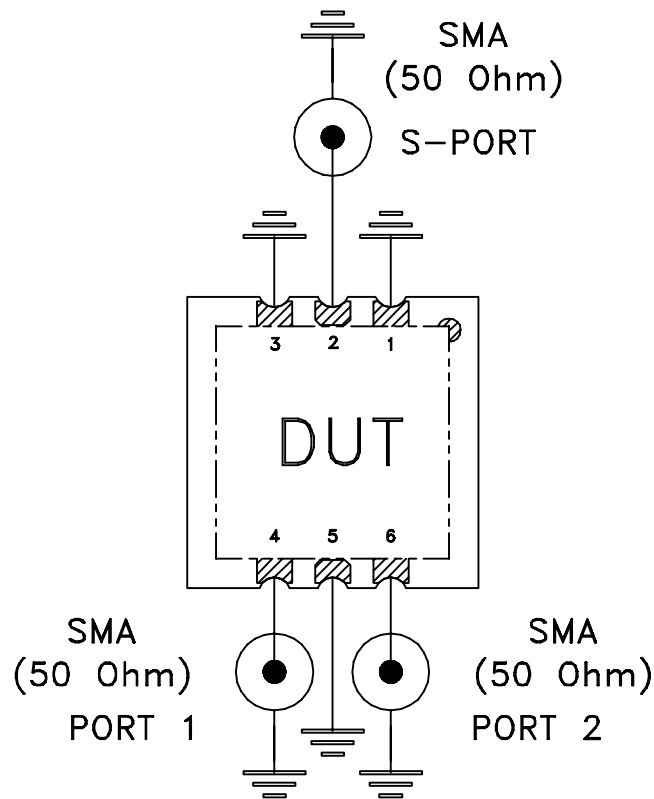
Schematic Diagram
