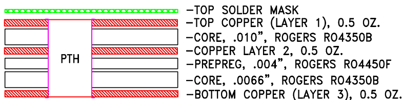
Stack-up Diagram
