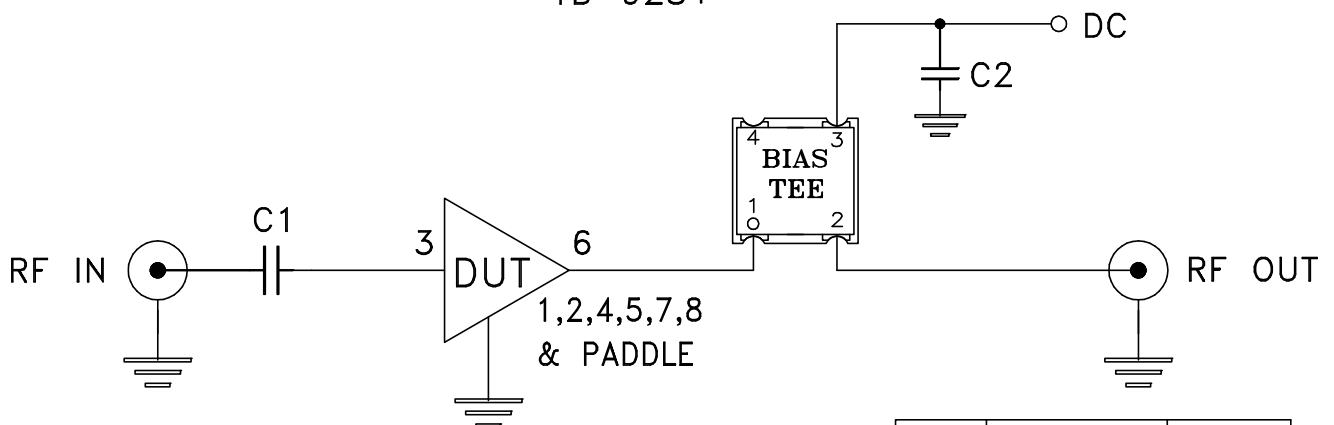
Schematic Diagram
