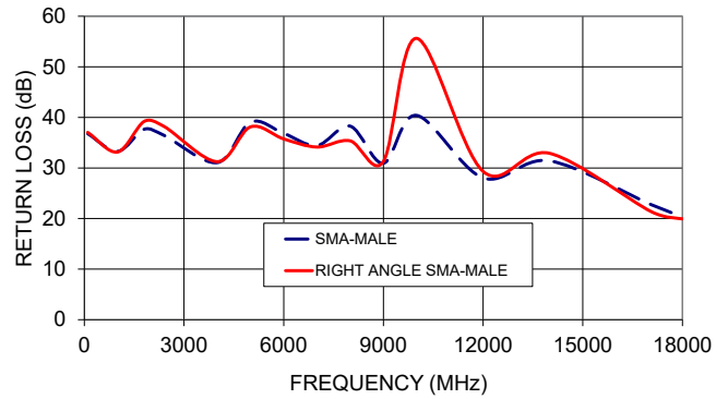
141-14SMRSM+ RETURN LOSS
