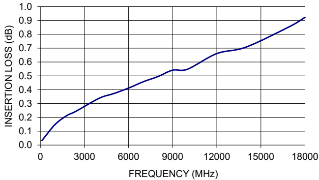
141-14SMRSM+ INSERTION LOSS
