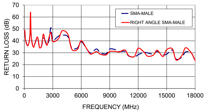
141-6SMRSM+ RETURN LOSS
