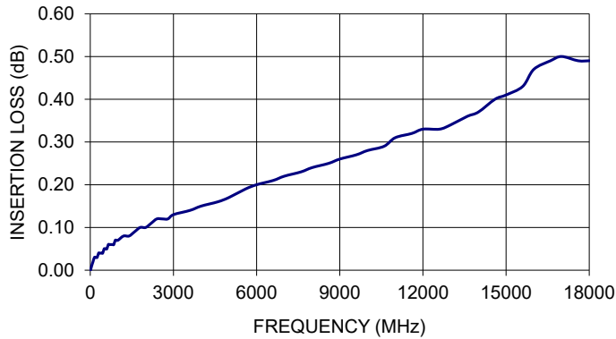
141-6SMRSM+ INSERTION LOSS
