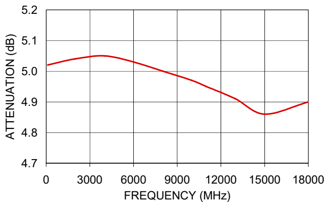
BW-N5W5+ ATTENUATION
