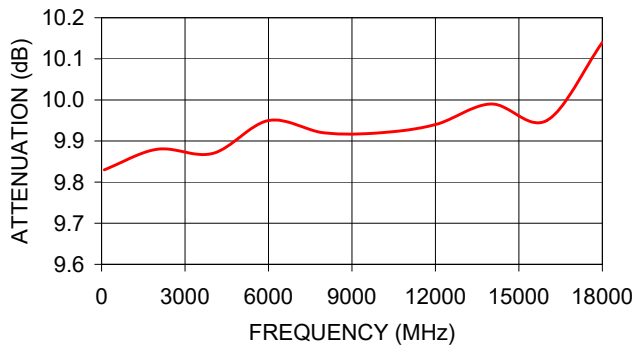
BW-S10W5+ ATTENUATION
