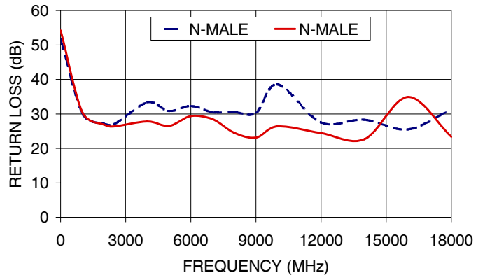
CBL-1.5M-NMNM+ RETURN LOSS
