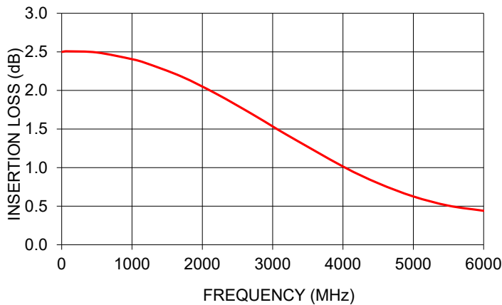
EQY-2-63+ INSERTION LOSS
