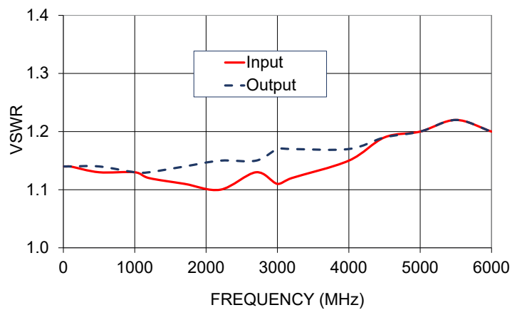
EQY-8-63+ VSWR
